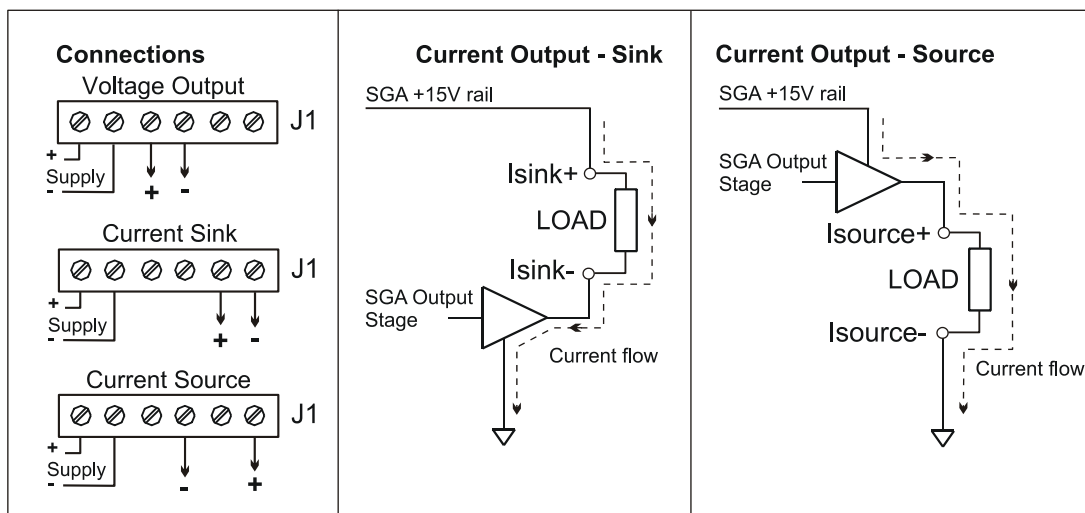
Figure 2.5 Output Connections
